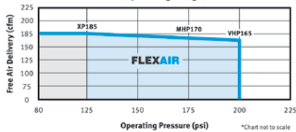
XP185-VHP165 Variable Flow and Pressure (Operating Range)
