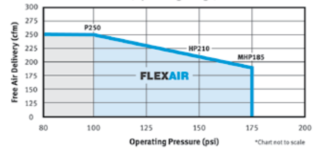
P250-MHP185 Variable Flow and Pressure (Operating Range)
