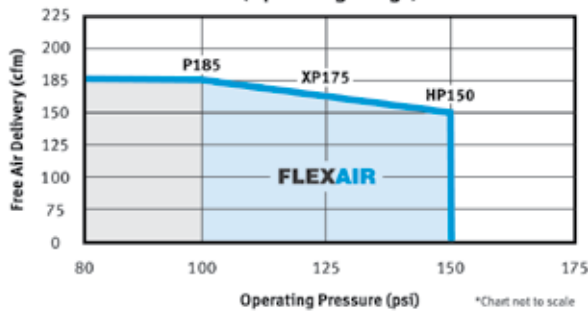
P185-HP150 Variable Flow and Pressure (Operating Range)
